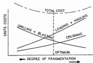
Fig-4 Optimum fragmentation
