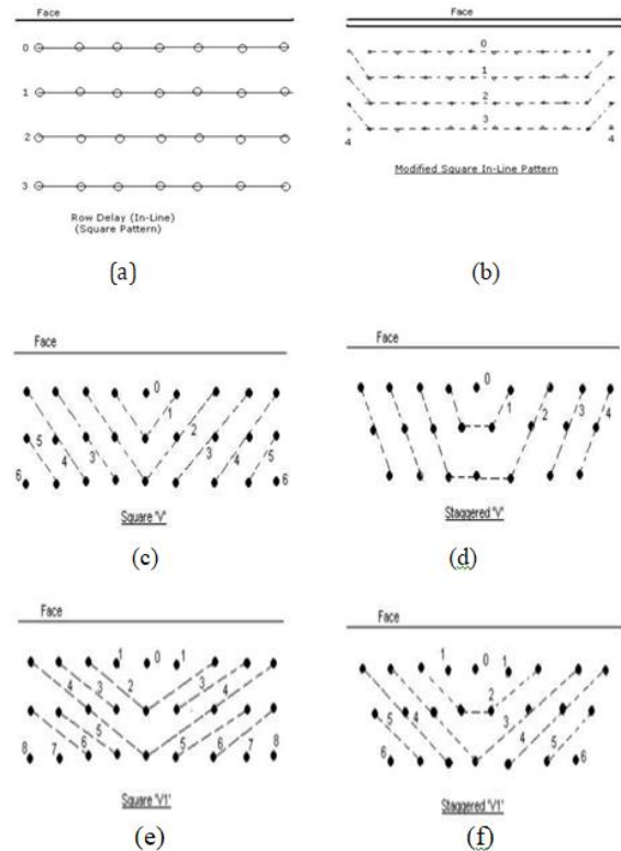
Fig-3 Sequence of initiation in multi-row blasting
