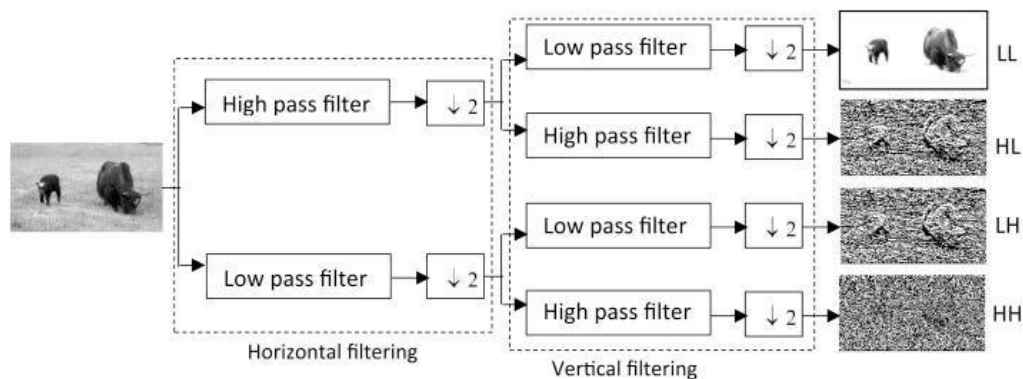
Figure 2. DWT decomposition.
