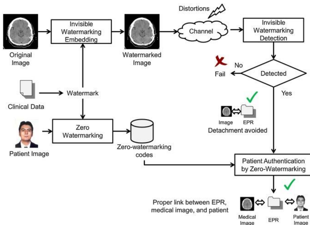
Figure 1: System architecture of proposed blind image watermarking system.
