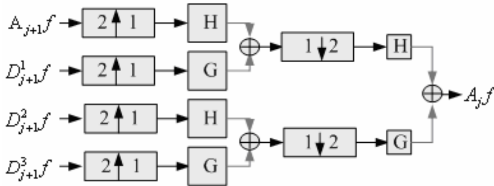
Figure 3. DWT reconstruction.
