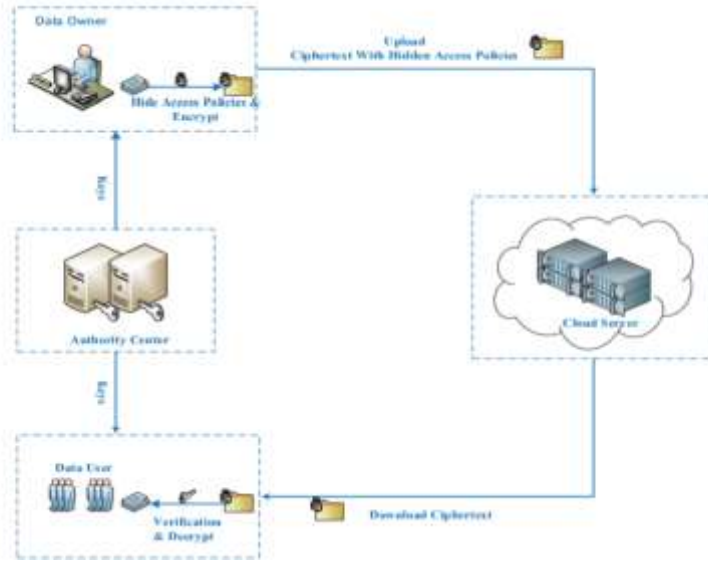
Fig 1: System Model
