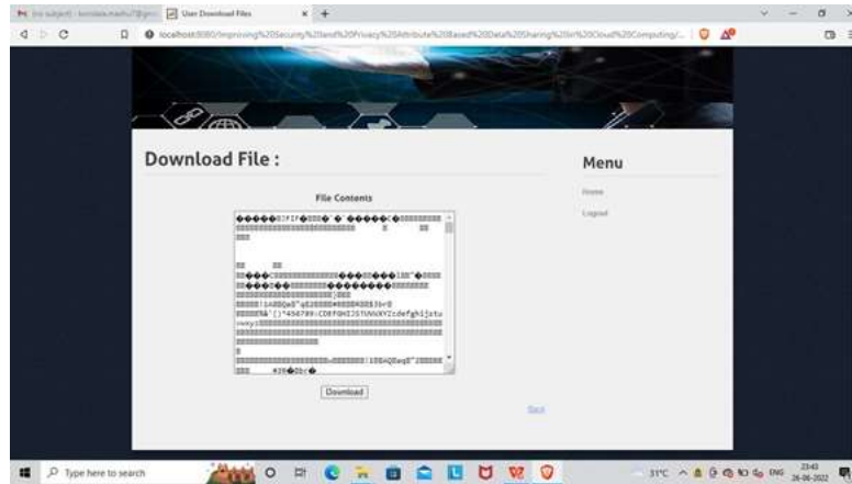
Fig 4.3 Decrypted Data
