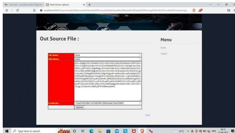
Fig 4.2 Encrypted Data
