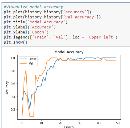
Fig 5: Accuracy cure
