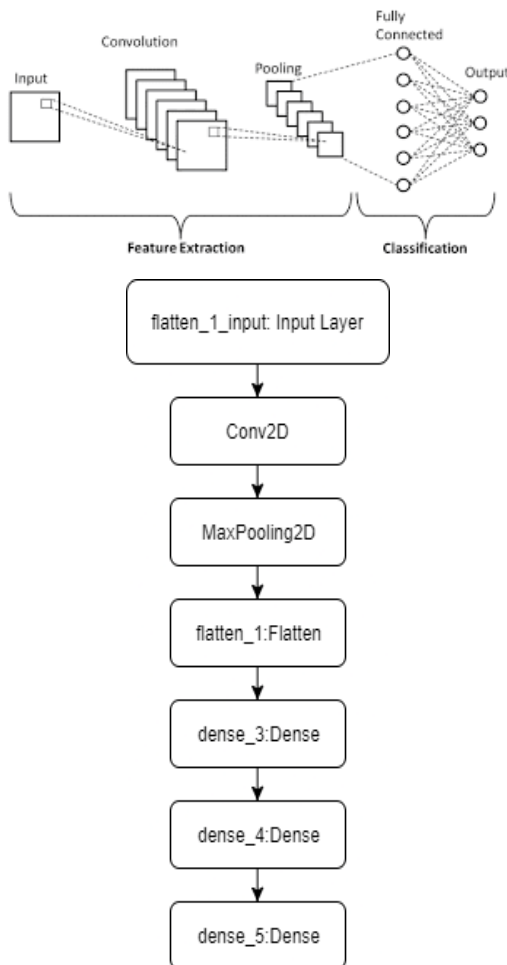
Fig 4: Simple
