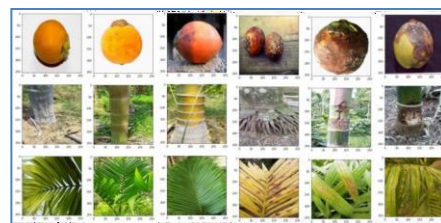
Fig 2: Sample dataset
