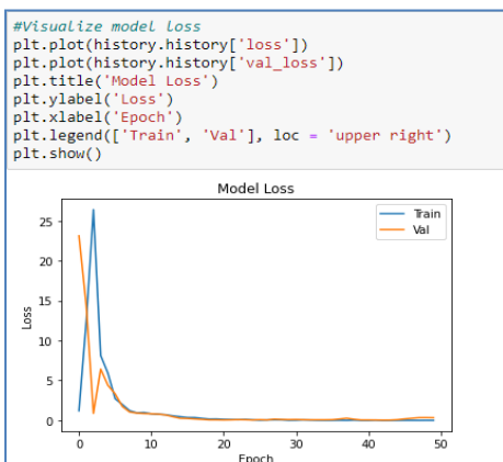
Fig 6: Loss cure
