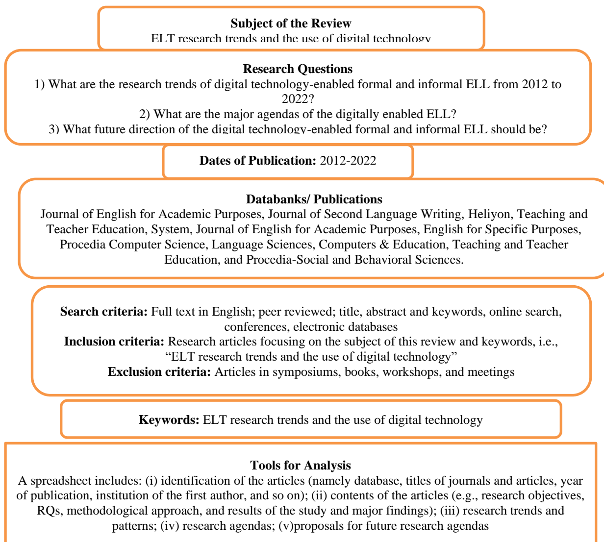
Figure 3 SLR protocol summary
