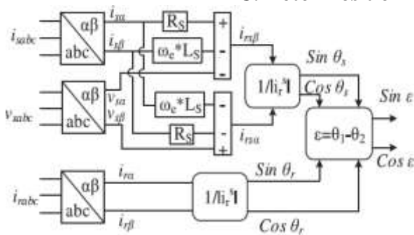
Fig. 4. Rotor position computation algorithm
