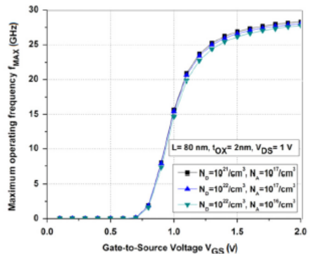
Figure 7. Maximum operating frequency (fMAX) as a function of gate-to-source voltage for various doping concentrations.
