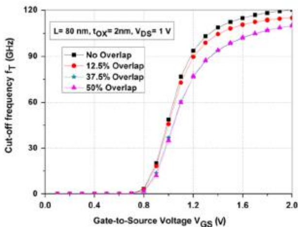
Figure 8. Unity-gain cut-off frequency fT as a function of gate-to-source voltage for gate underlap and overlap.
