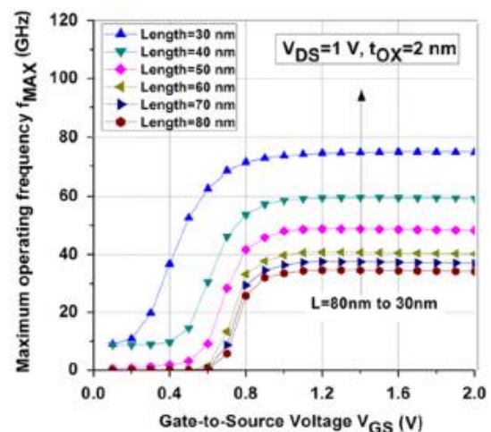
Figure 3. Maximum operating frequency f_{MAX} as a function of gateto-source voltage
