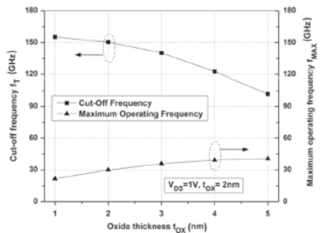
Figure 5. Unity-gain cut-off frequency (f T ) and maximum operating frequency (f MAX ) as a function of various oxide thickness t OX .
