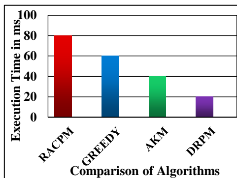
Figure 2. Execution time
