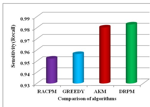
Figure 4. Sensitivity %
