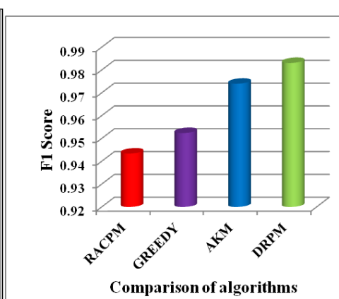
Figure 7. F1-Score %
