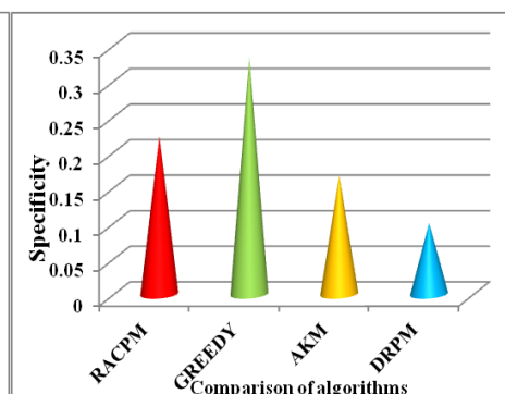
Figure 5. Specificity %
