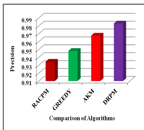
Figure 6. Precision %
