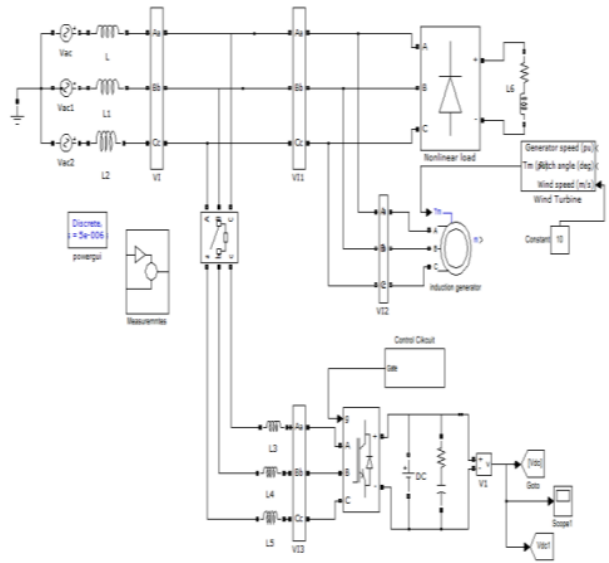
Fig.4: UPQC based wind non-linear load
