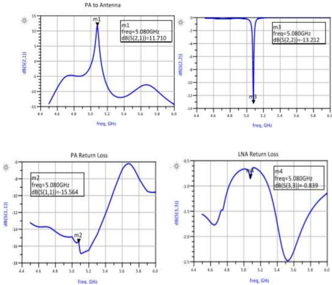
Fig.1: Results of RF transceiver antenna [89]
