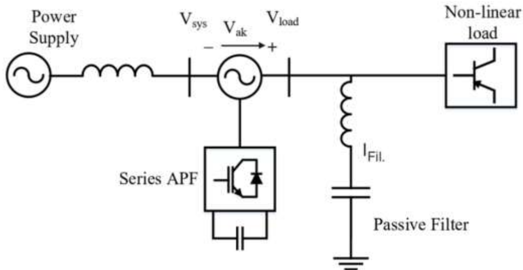
Fig 1 Series Connected VSC
