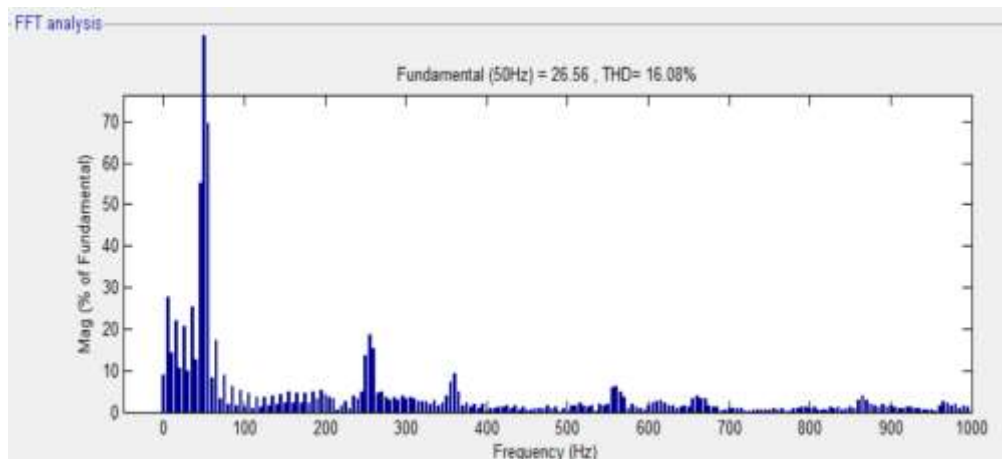
Fig 6 voltage THD profile before connecting proposed system
