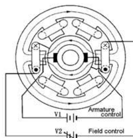
Figure 8: Cross-sectional View of DC Motor
