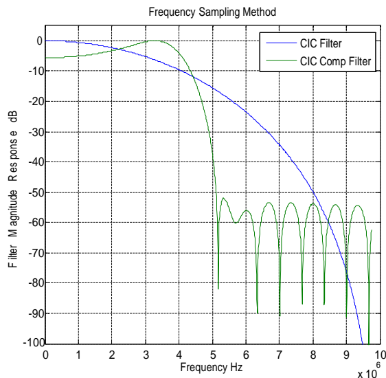
Fig 5- Response of CIC compensation filter
