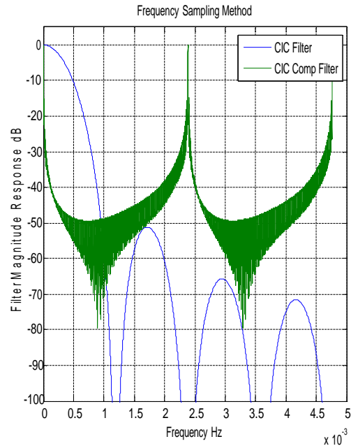
Fig 6. Final response of Compensation filter
