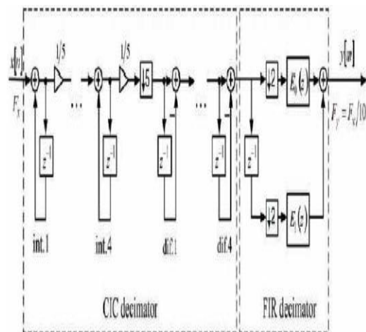
Fig-3 compensation filter
