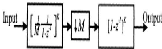
Fig.1 CIC filter
