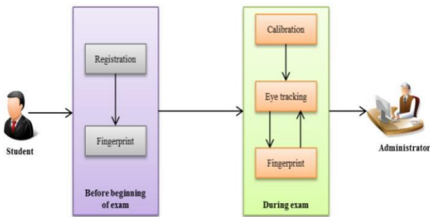
Figure II.1 E-Exam Architecture [10]
