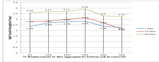
Graph No. – 3 Split-Tensile strength test results
