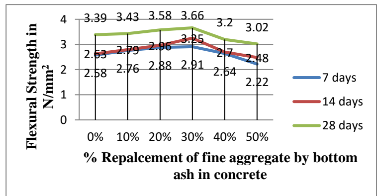
Graph No. – 4 Flexural strength test results
