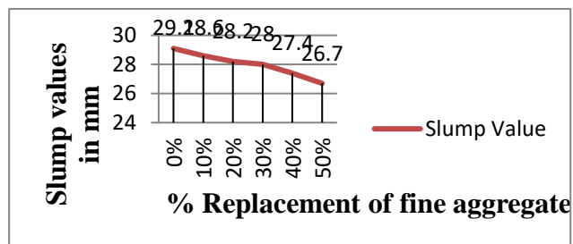
Graph No. - 1 Slump cone test results
