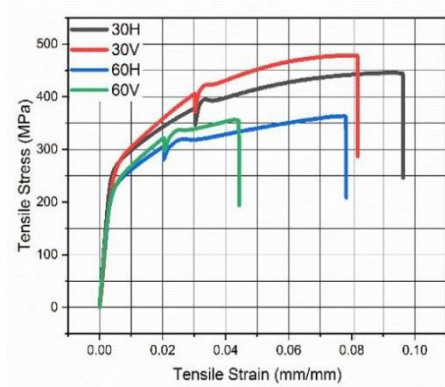
Figure 6: Tensile test results plot different layer thickness and build direction
