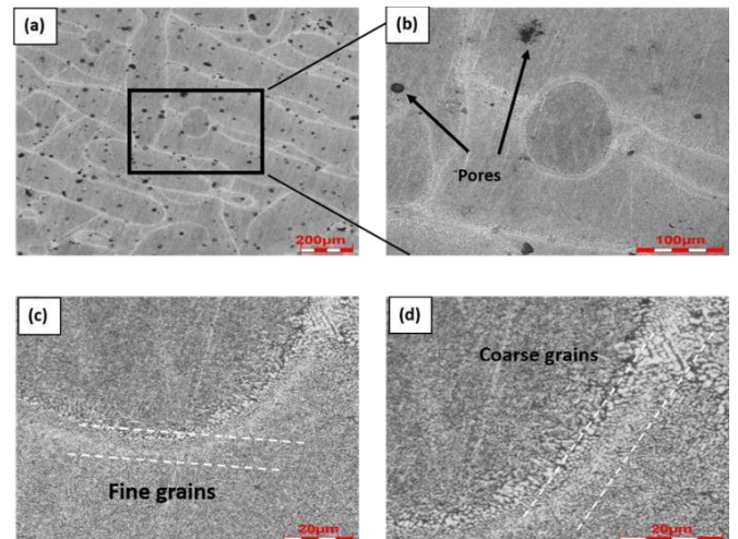
Figure 4. Optical images of AlSi10Mg @ 60 \mu m layer thickness (a) microstructure @ 200X (b) Microstructure @ 693X magnification and (c) Microstructure @ 2000X magnification (d) microstructure @ 4000X
