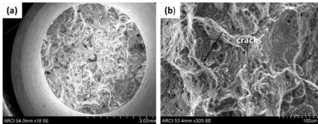
Fig 9. SEM fractography micrographs of 60µm vertical built
