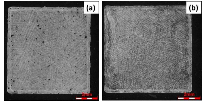
Figure 3. Top view of micro structure of AM built AlSi10Mg (a) 60 \mu m (b) 30 \mu m
