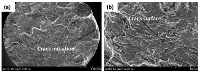
Fig 8. SEM fractography micrographs of 30µm horizontal built
