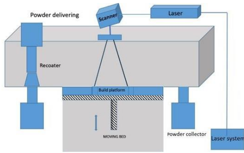
Figure 1. Schematic diagram of SLM
