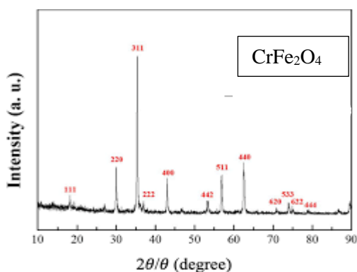
Fig.1: X-ray (XRD) pattern of CrFe 2 O 4 nanoparticles.
