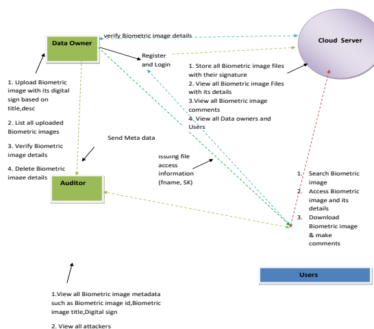
Architecture Diagram
