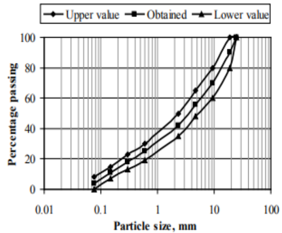
Figure: 3.3..Grain size distribution of aggregate gradation
