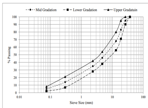
Graph:3.1. Aggregate Gradation of Bituminous Concrete (BC) mix
