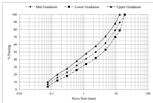
Graph:3.1. Aggregate Gradation of Bituminous Concrete (BC) mix
