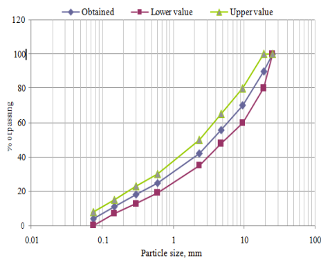
Graph:3.3. Grain size distribution of aggregate gradation
