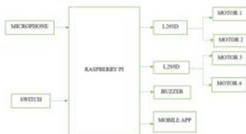
Figure 2: Block Diagram
