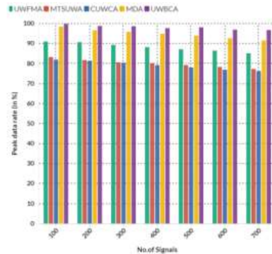
Fig.4. Comparison of Peak data rate
