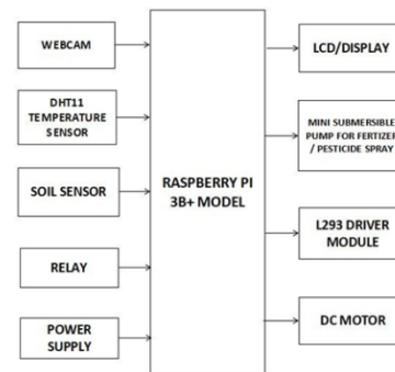
Figure.1: Block Diagram
