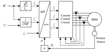
Fig. 5. Vector control system for SRM drive.
