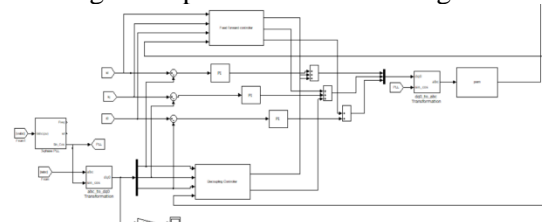
Fig7: Control Design
